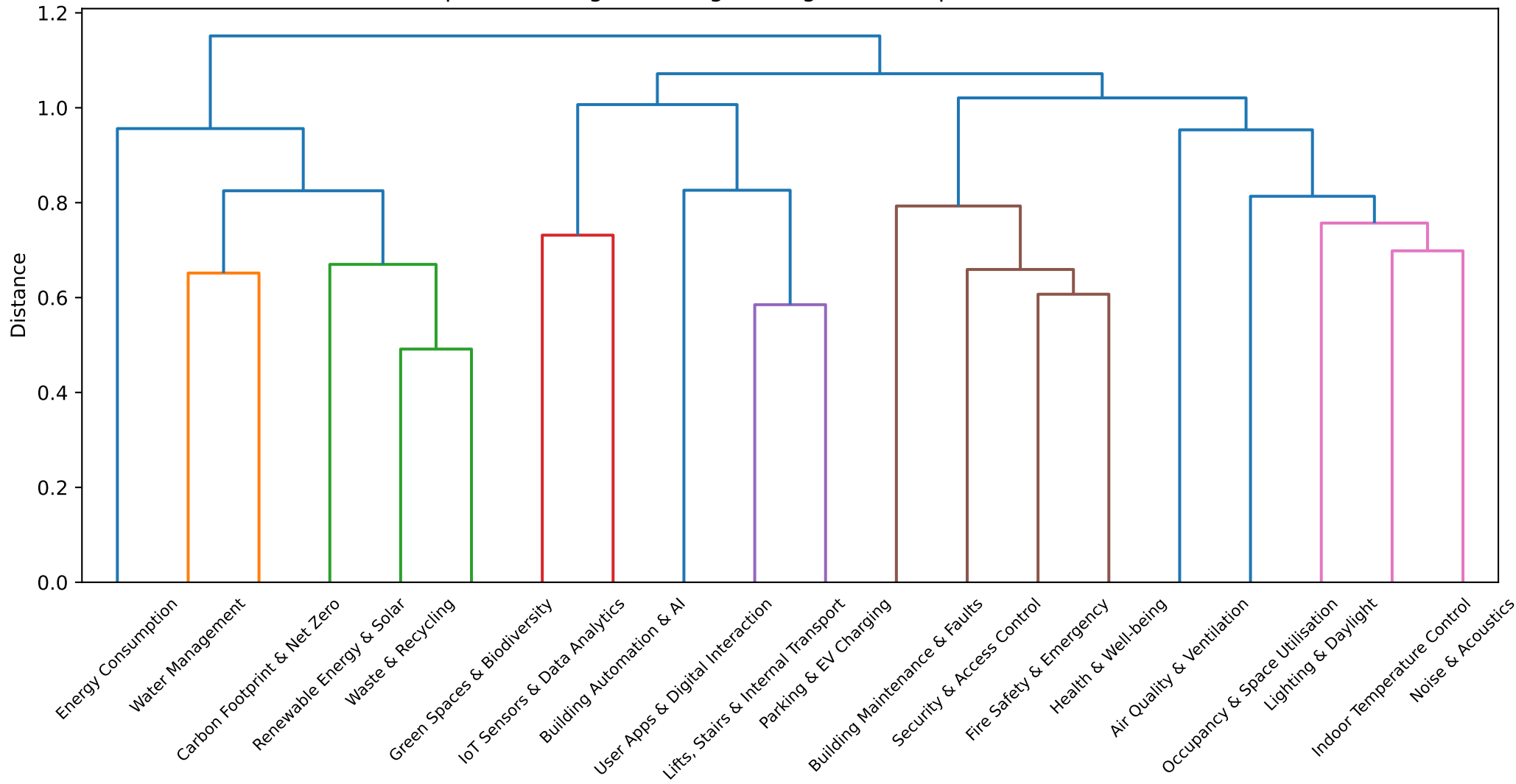
Topic clustering — average linkage on (1 - Spearman) distance
